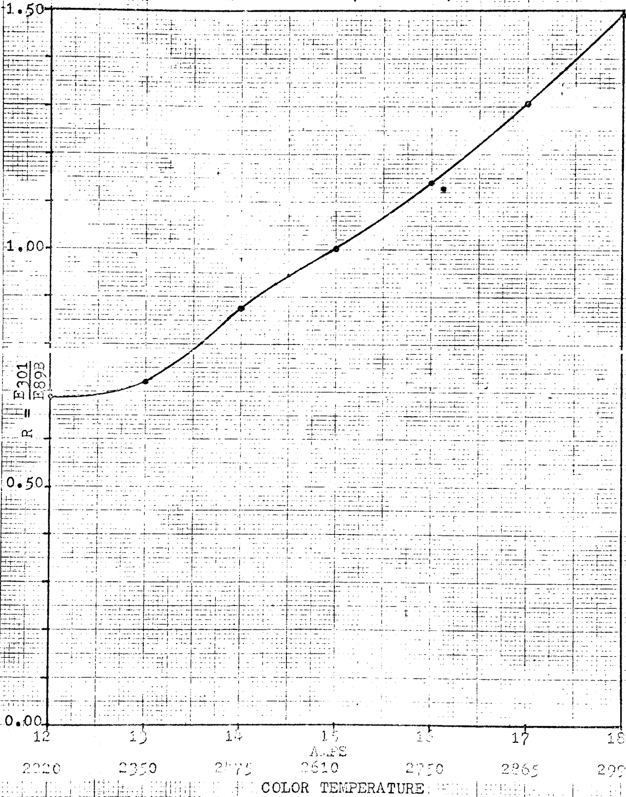
FIG. 16. CALIBRATION CURVE (R vs AMPS)
