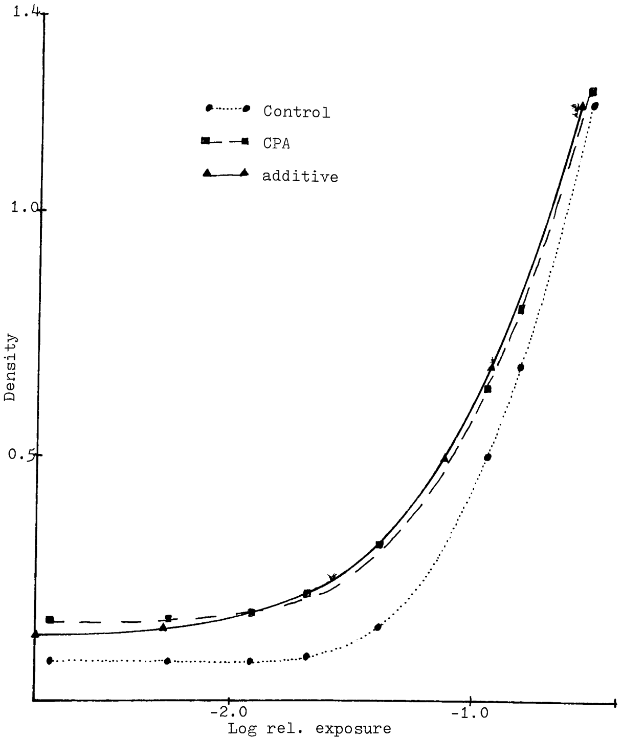
Fig. 15. Density as a function of exposure with supplementary exposure -1.45 \text{ Log rel.H} corresponding to .05 over B+F.
