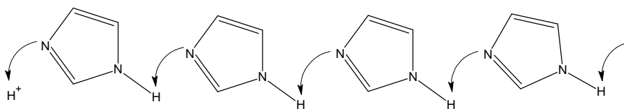
Figure 10. Grötthus mechanism of proton transport through imidazole molecules
