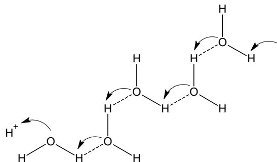
Figure 9. Grötthus mechanism of proton transport through water molecules
