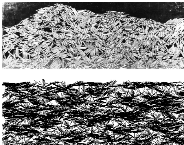
FIG. 1. Top: 2D pile of \alpha=12 acrylic rods backlit with fluorescent lights. The middle third of each particle appears bright. Bottom: Simulated pile of \alpha=12 particles. Both piles show particles aligning and a wide distribution of void sizes.
