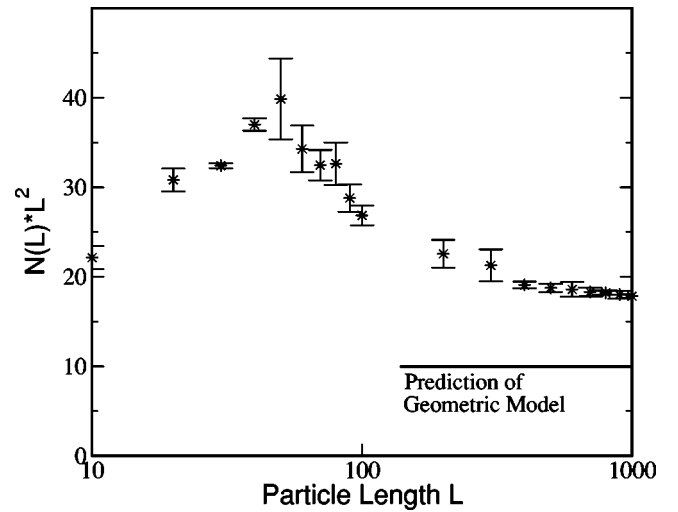
FIG. 9. Number density multiplied by L^2 as a function of particle length. As predicted by the simple geometric model described in text, the number density appears to scale as L^{-2} for large L . The actual densities, however, are larger than that predicted by the model, a consequence of particle alignment.
