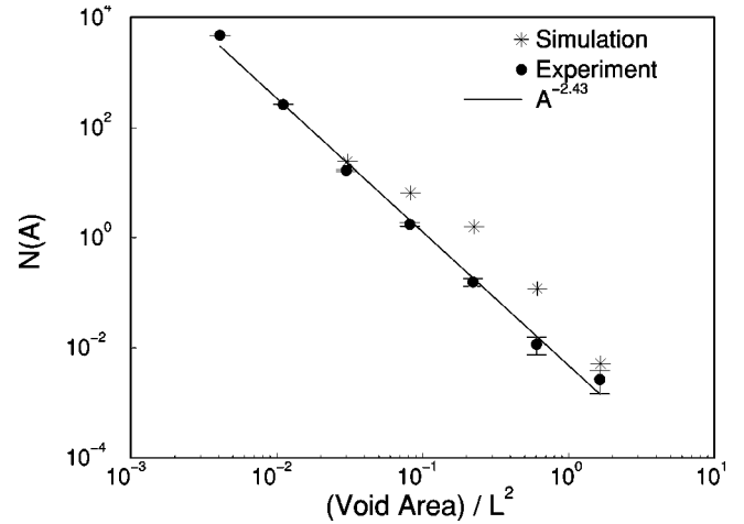
FIG. 5. Void distribution function N(A) as a function of dimensionless void area (area scaled by particle length L squared). Voids in experimental piles (●) decay as a A^{-\beta} with \beta=2.43 \pm 0.08 . Simulations (*, with \alpha=20 ) show a similar decay, though not strictly a power law. The exponent's value means that smaller voids occupy a greater total area than the larger, rarer, voids.
