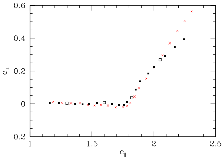
Fig. 19.— As Figure 18, but the axes have been rotated to the c_{\parallel}-c_{\perp} system.
