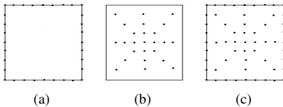
Fig. 2. Key points models. (a) key points sampled from the bounding box sides, (b) key points sampled evenly from the diagonals, horizontal and vertical center lines, and (c) key points from both the bounding box interior and sides
