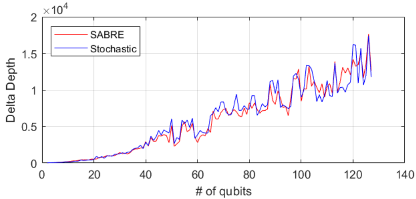
(b) Depth - SABRE v. Stochastic
