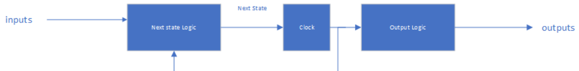
Figure 3.3: Moore Machine
