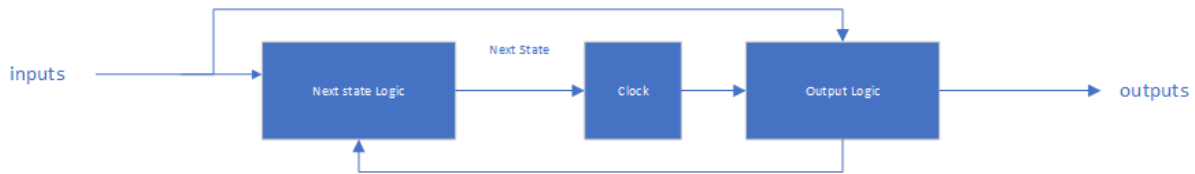
Figure 3.2: Mealy Machine
