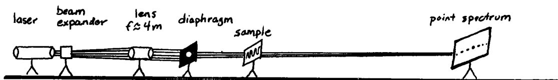
Laser set-up Figure 6
