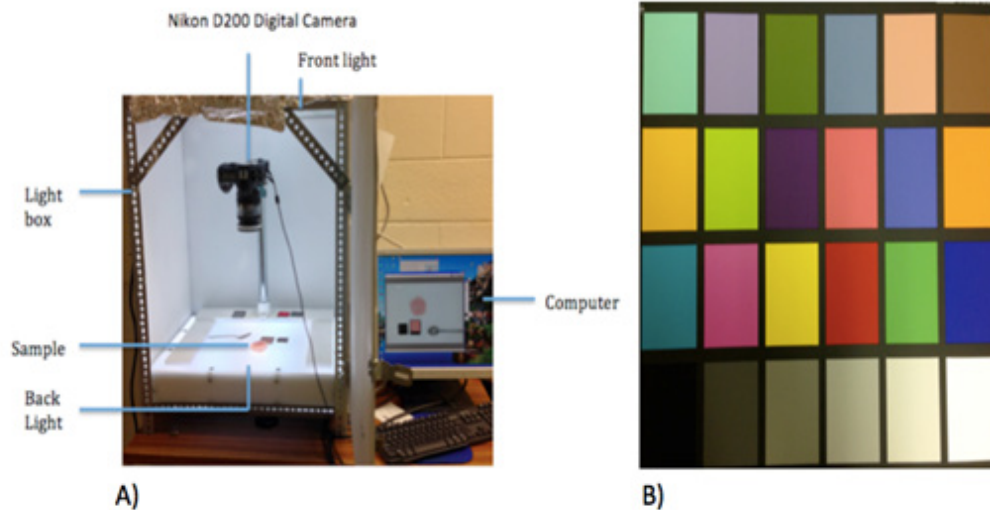
Figure 3. Machine Vision System. A) photograph of the system of machine vision, B) the color chart was used in the calibration process as references.
